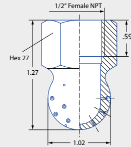
Female thread
