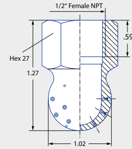
Female thread
