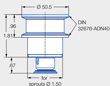
Tri-Clamp connection
